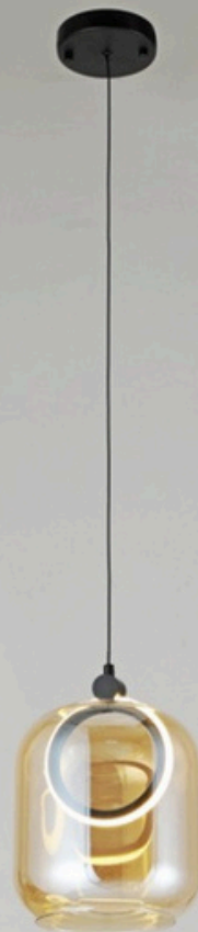
Item No : 2328 Lamp : Led Size : D220MM X FH260MM Finish : Black Material : Metal + Glass + Silicone
